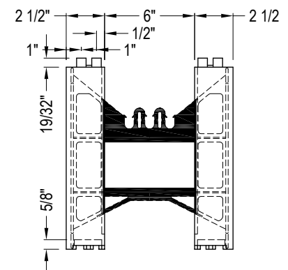
CORNER BLOCK TYPICAL SECTION DETAIL
